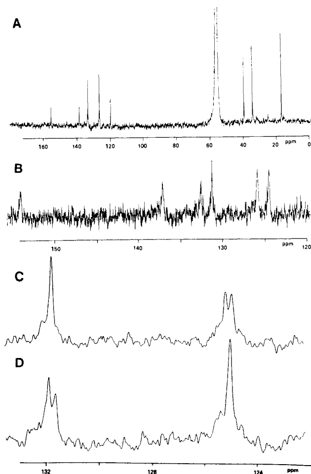
Figure 3. Low-temperature ( -60\ ^\circ\text{C} ) 125-MHz spectra of TPrP in \text{CD}_2\text{Cl}_2 . (A) Proton decoupled spectrum, 3000 scans. (B) Proton coupled spectrum of the pyrrole region ( \alpha and \beta carbons), 25000 scans. (C) Carbon spectrum recorded with single frequency decoupling at 9.49 ppm ( \beta hydrogens of the \alpha -pyrroline like ring), 1000 scans. (D) Same as spectrum C, obtained by decoupling of the hydrogens appearing at 9.60 ppm.
